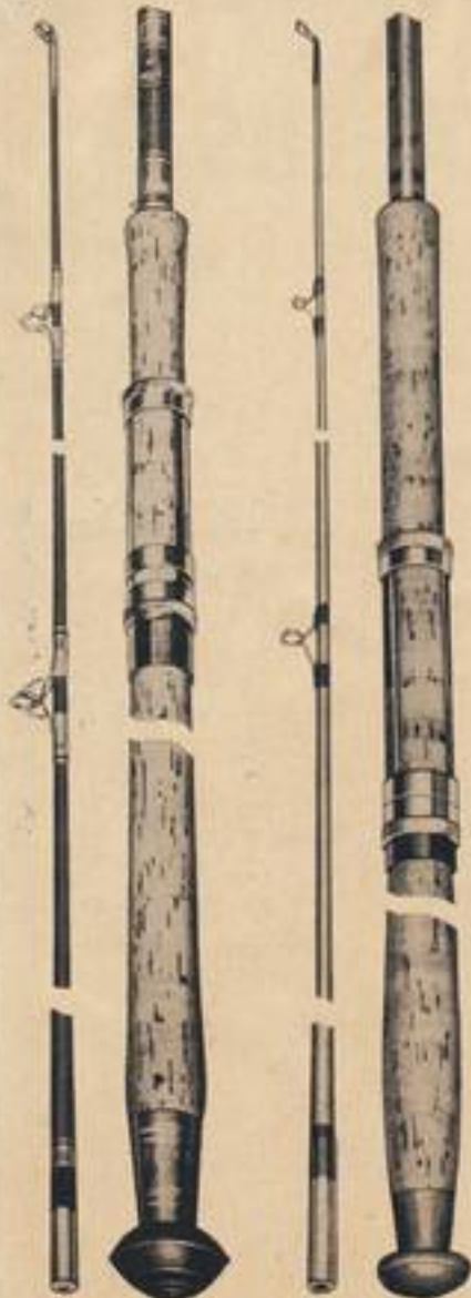
Gulf Stream
